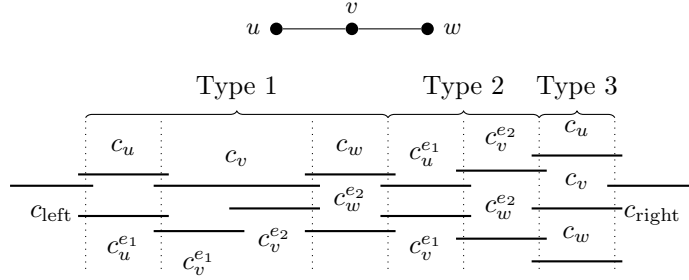
Figure 1: A graph, and the set of intervals obtained by applying the reduction used in the proof of Theorem 2.2 when k = 2 .
